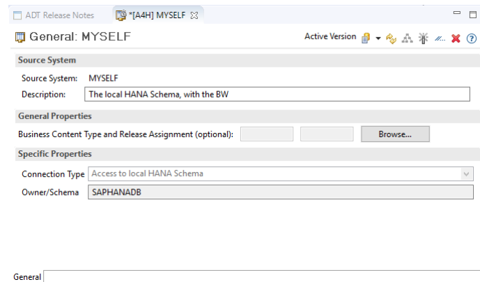
Figure 2: Properties of the Source System MYSELF
